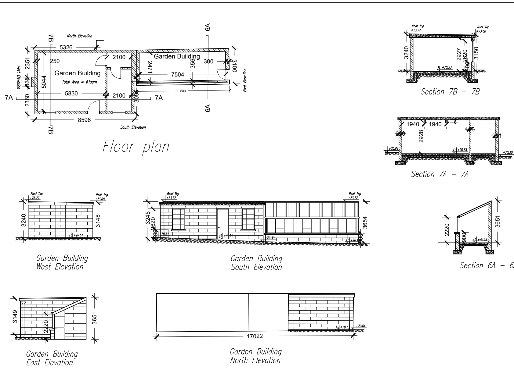
Existing Garden Buildings Scale 1:200 @ A3
